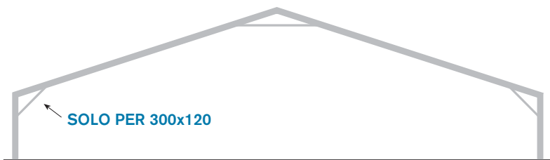
Capriata intermedia
